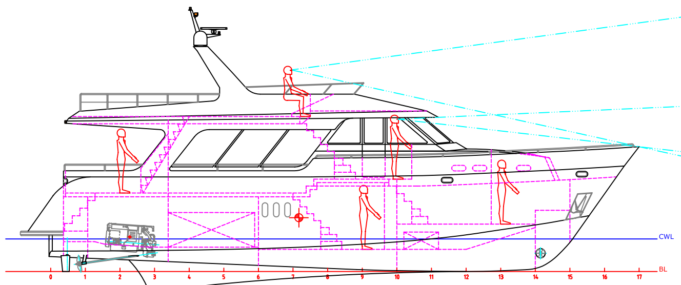
Flying-bridge
